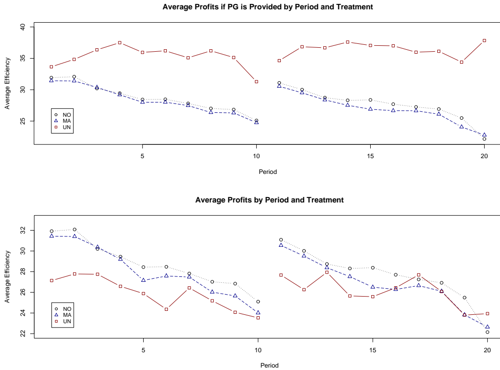
Figure 3: Average profits
